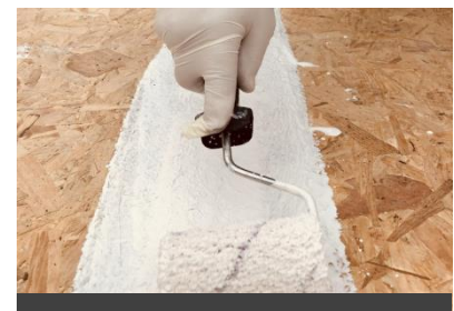
Square edge OSB3 joints reinforced with primer and taping
